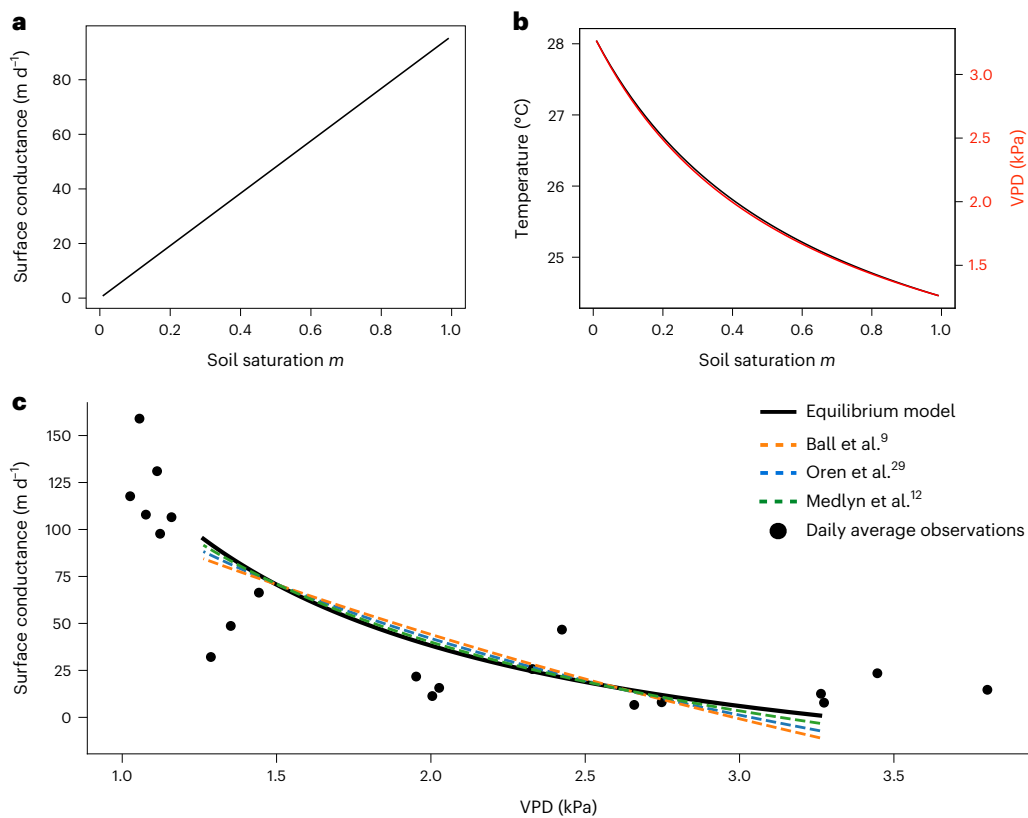
Fig. 3 | Surface conductance in the equilibrium model. a , The relation between surface conductance and soil moisture parameterized into the equilibrium model. b , The relations among atmospheric potential temperature, atmospheric VPD and soil moisture output from the equilibrium model. c , The emergent
